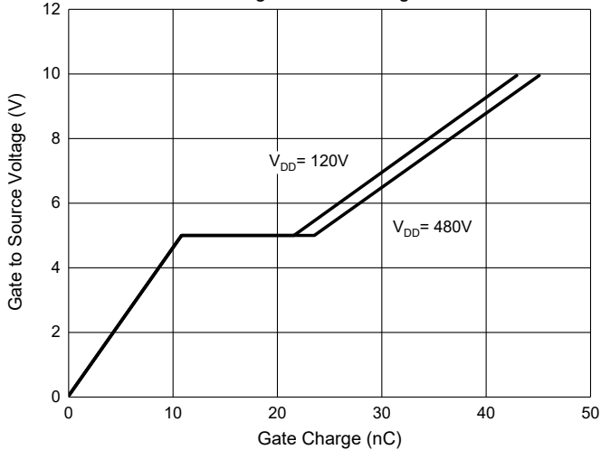
Fig. 5 - Gate Charge
